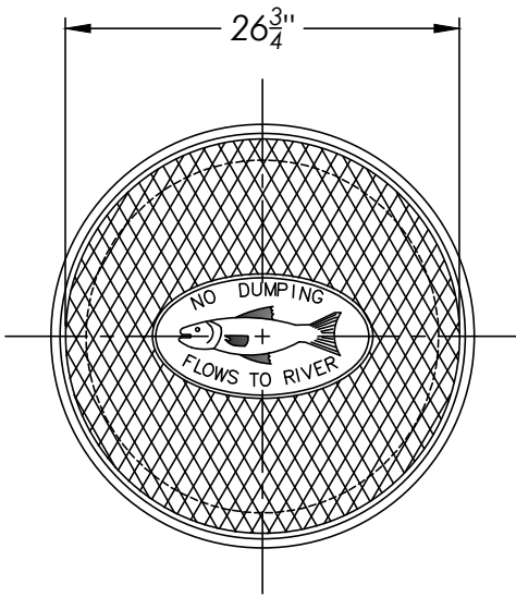
(A) CAST IRON COVER
