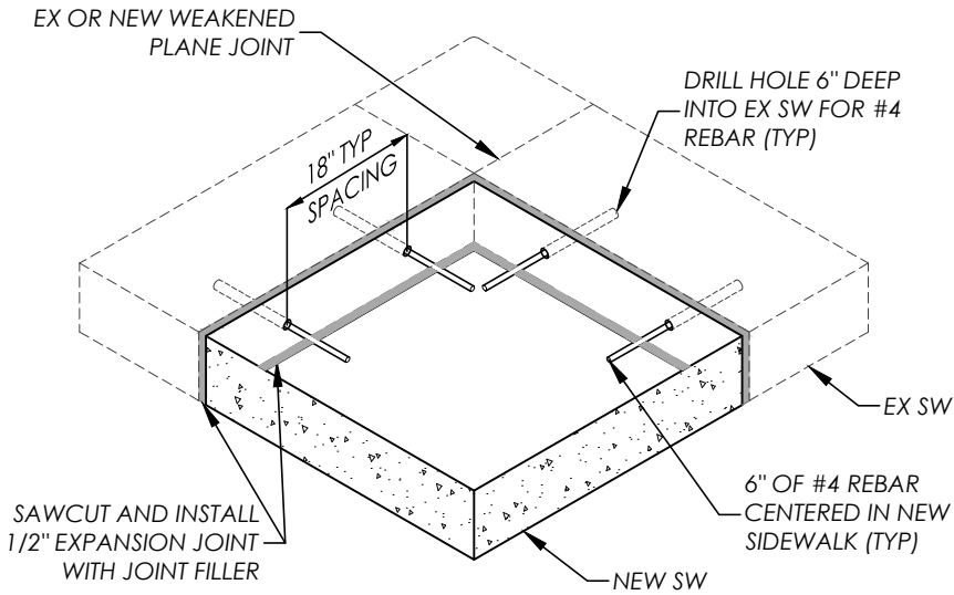
SIDEWALK CONNECTION
