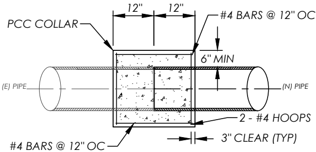
CONCRETE COLLAR CONNECTION
