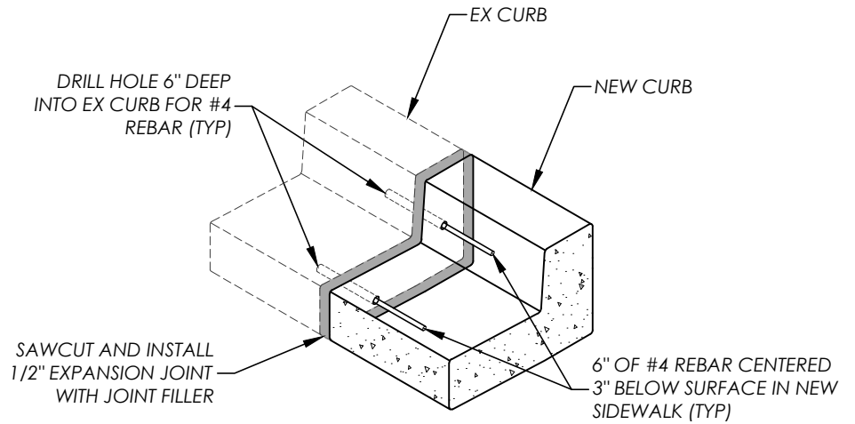
CURB AND GUTTER CONNECTION
