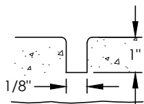
TYP. WEAK PLANE JOINT
