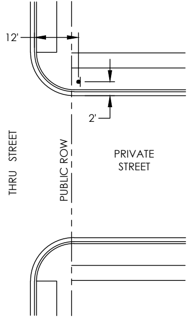
ALT. "A" LOCATION ON CURB RETURN
