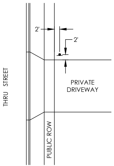
ALT. "B" LOCATION ON DRIVEWAY APPROACH
