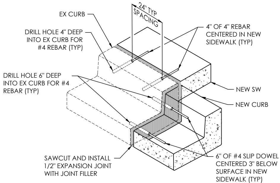
SIDEWALK, CURB AND GUTTER CONNECTION
