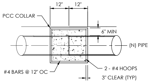
CONCRETE COLLAR CONNECTION
