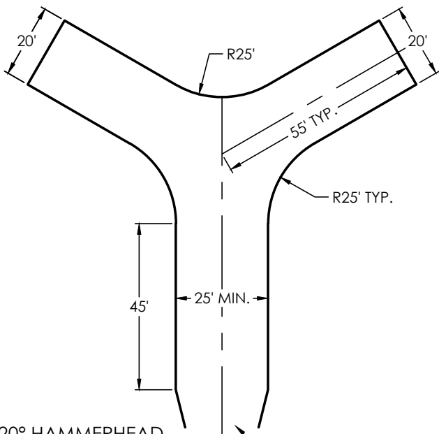
120° HAMMERHEAD (NO PARKING)
