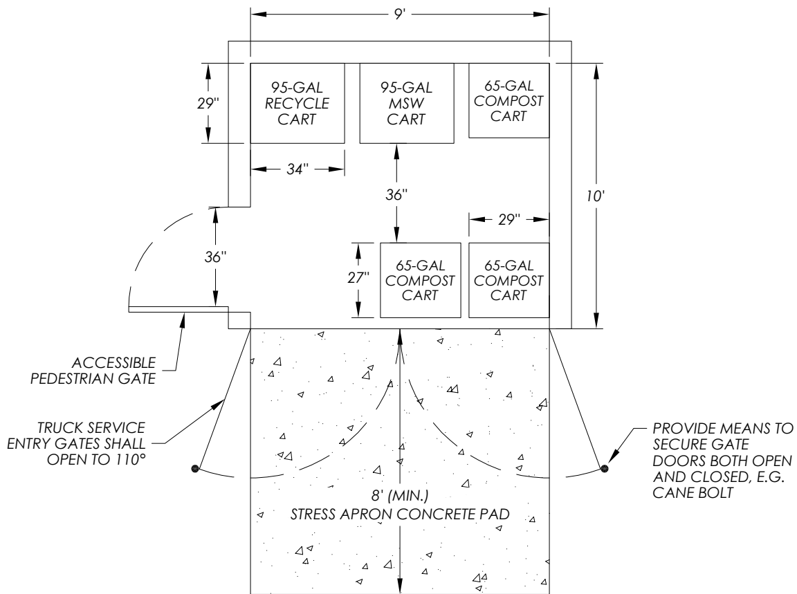
PLAN VIEW
