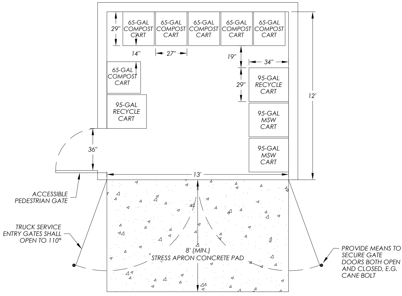
PLAN VIEW
