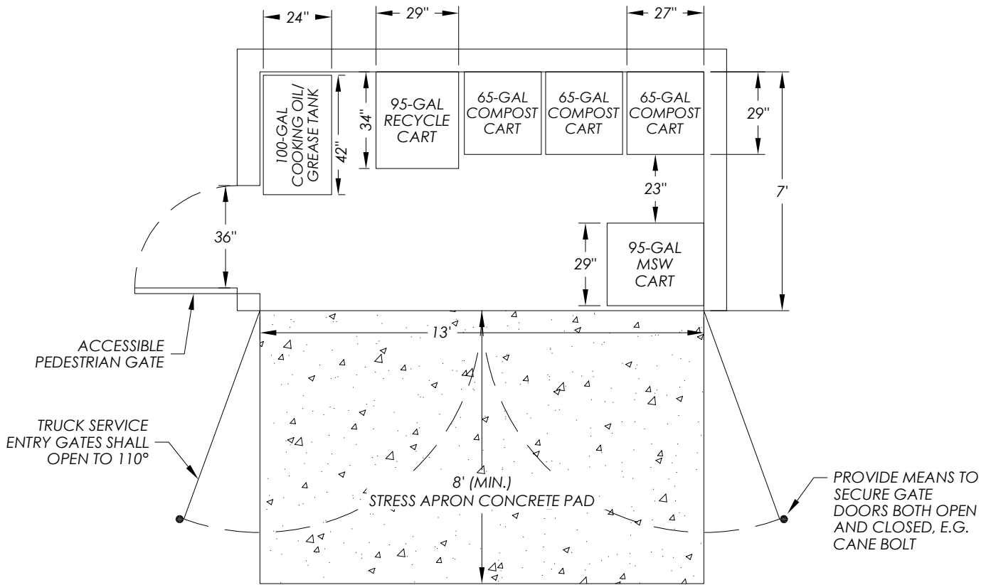
PLAN VIEW
